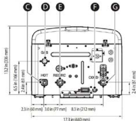
SupplyConnections
